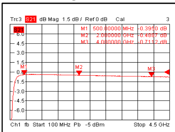
Insertion Loss @+85°C
