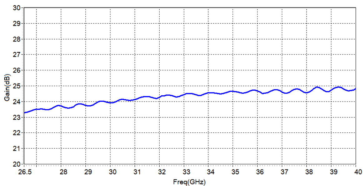
OLB-28-25-28319007-Gain(3m)
