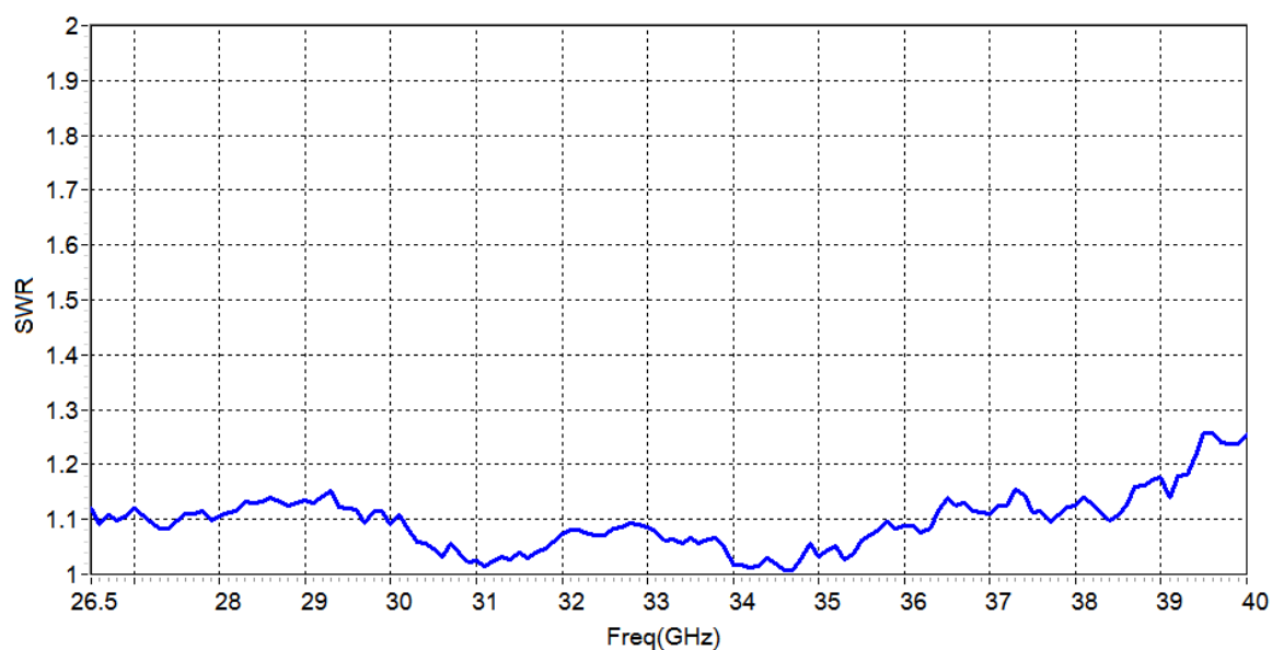
OLB-28-25-28319007-SWR
