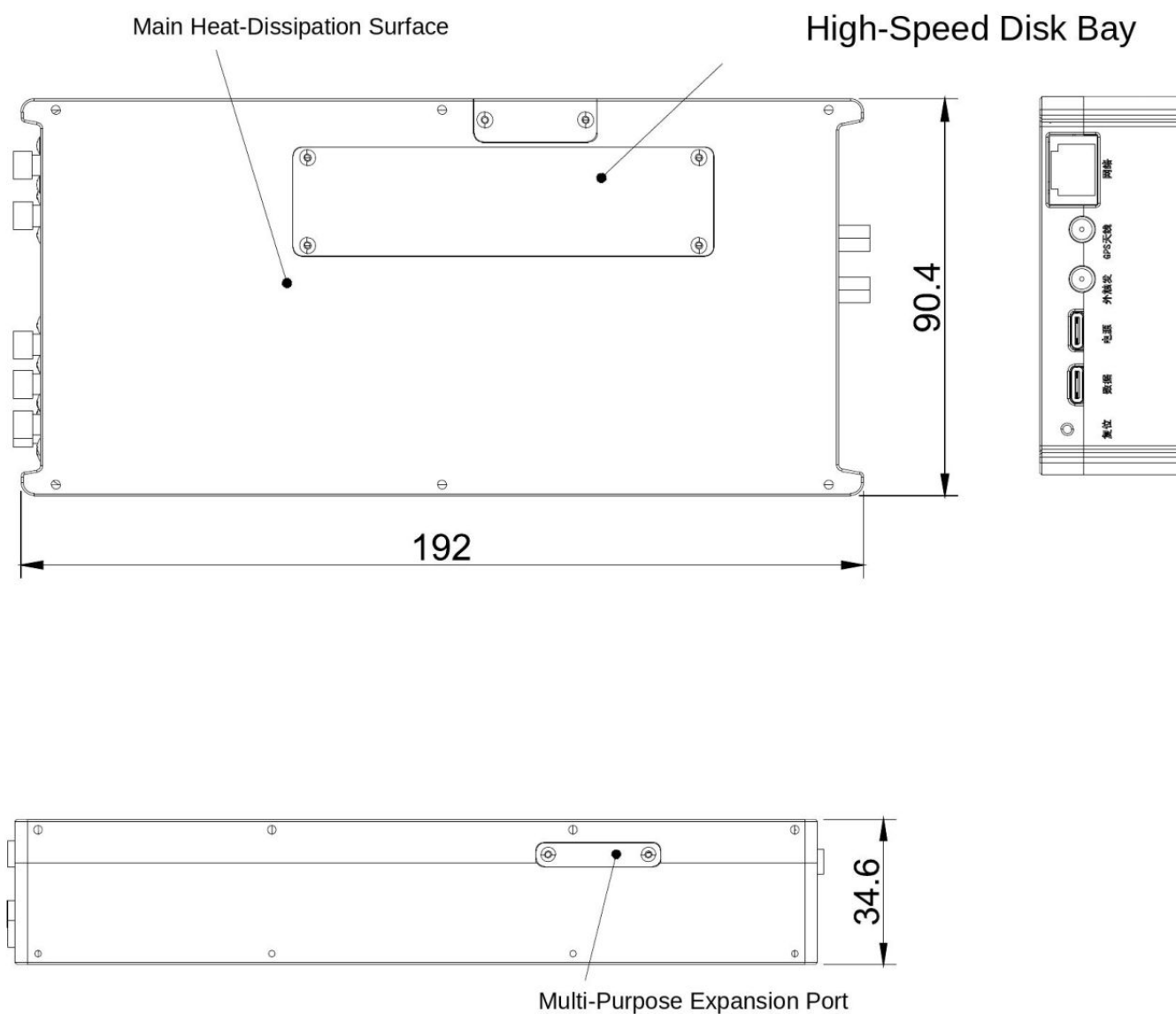
Mechanical outline drawing
