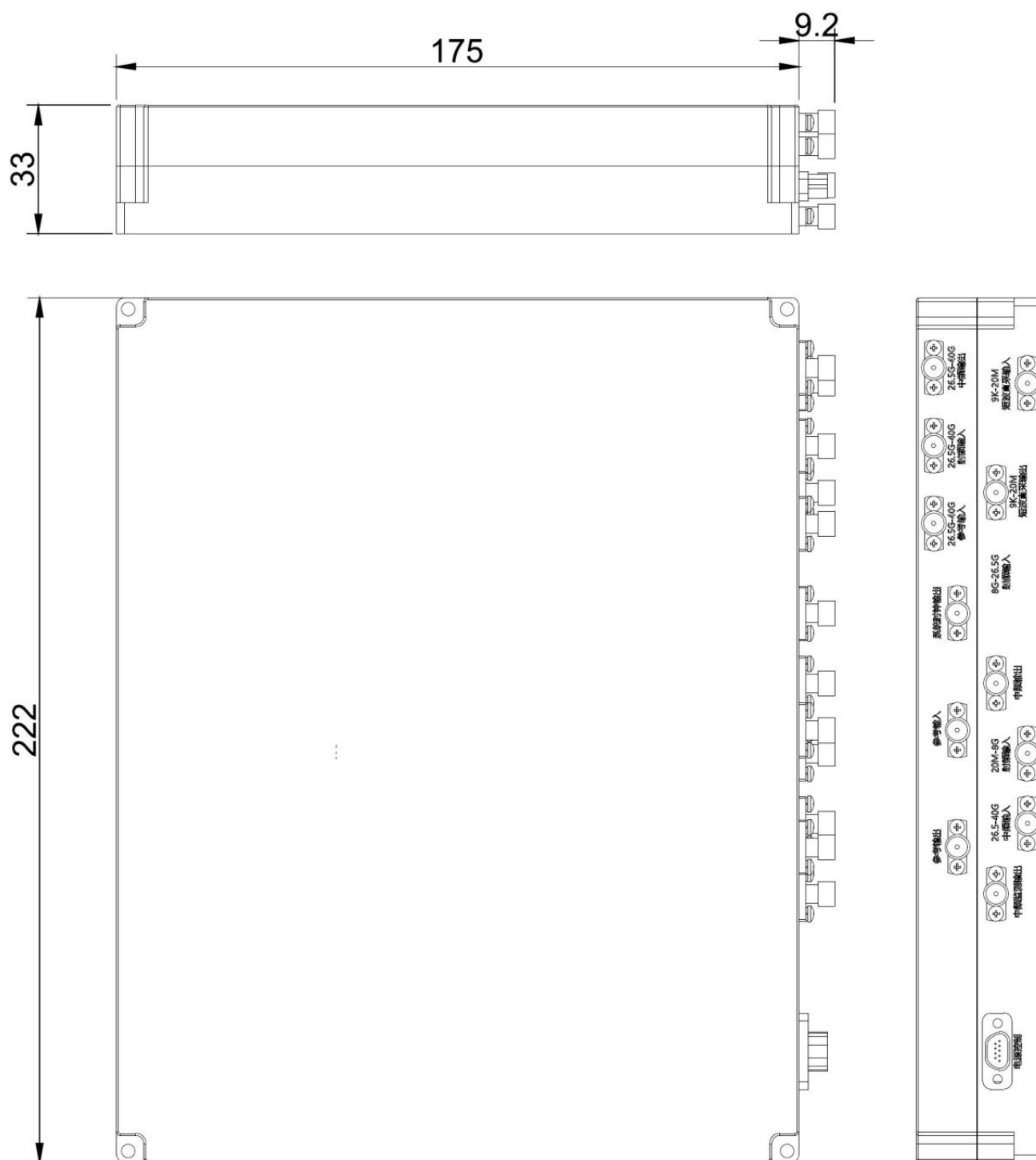
RF receiver module outline
