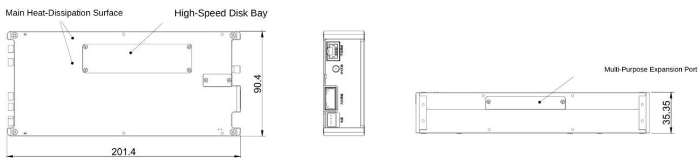
Mechanical outline drawing
