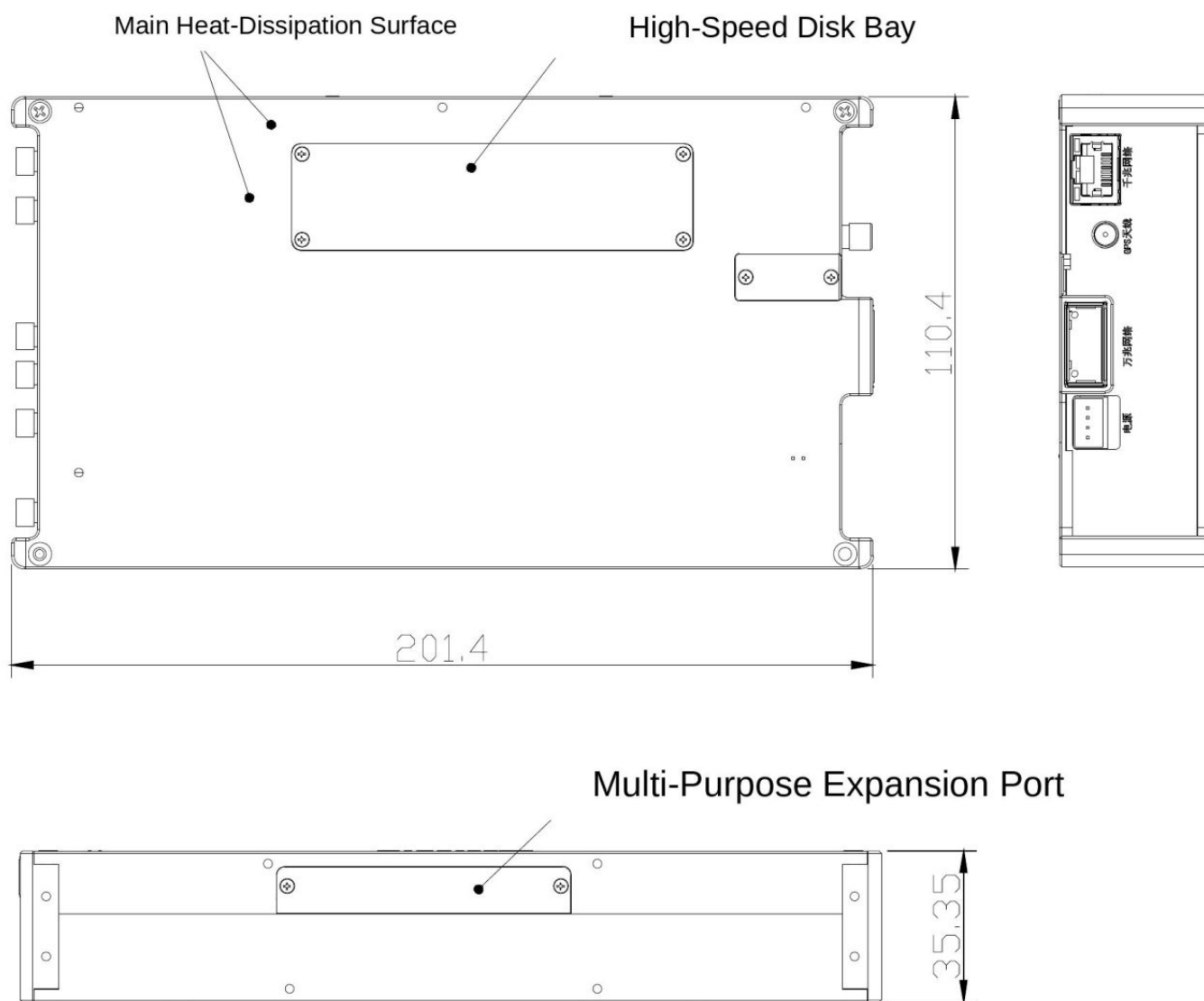
Mechanical outline drawing
