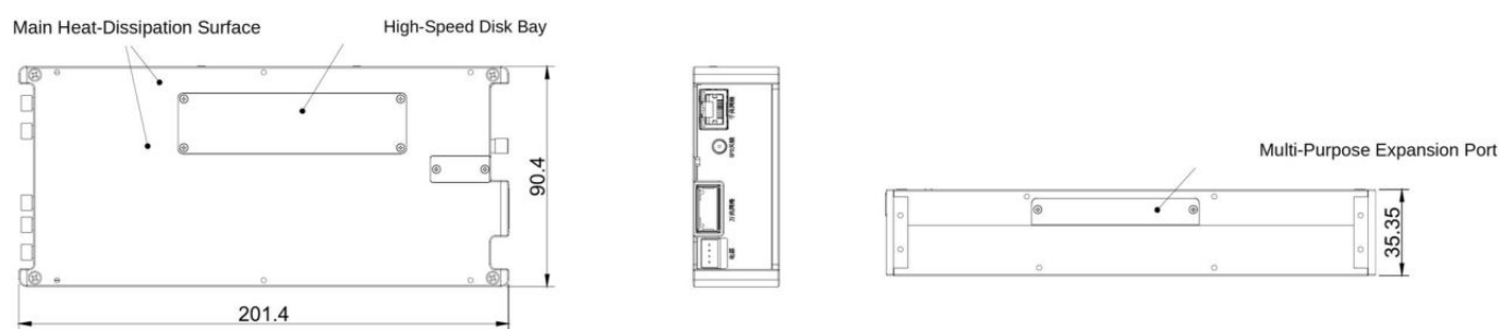
Mechanical outline drawing
