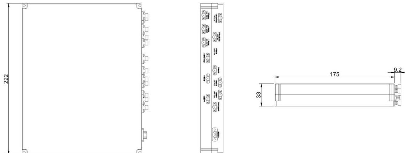
RF receiver module outline
