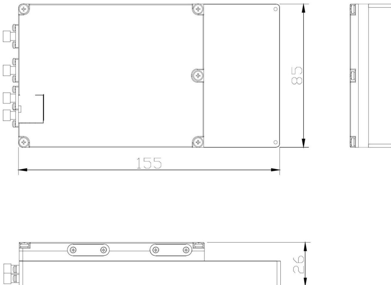
Mechanical outline drawing
