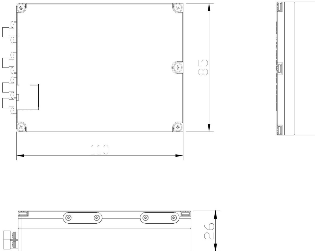
Mechanical outline drawing
